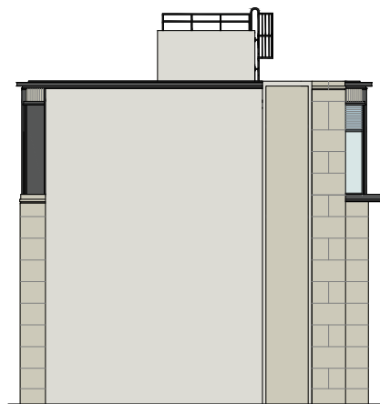
Elevation Plan D 立面圖 D (For Villa 30 Only) (僅限30號洋房)
