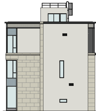
Elevation Plan D 立面圖 D (For Villa 8 to 12 & 16 Only) (僅限8至12及16號洋房)
