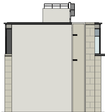
Elevation Plan D 立面圖 D (For Villa 19 Only) (僅限19號洋房)
