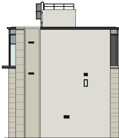
Elevation Plan C 立面圖 C (For Villa 9 to 12 Only) (僅限9至12號洋房)
