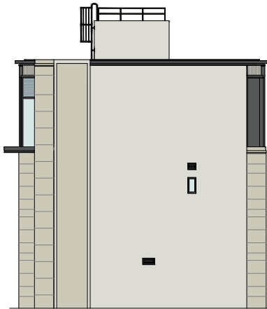
Elevation Plan C 立面圖 C (For Villa 8 Only) (僅限8號洋房)
