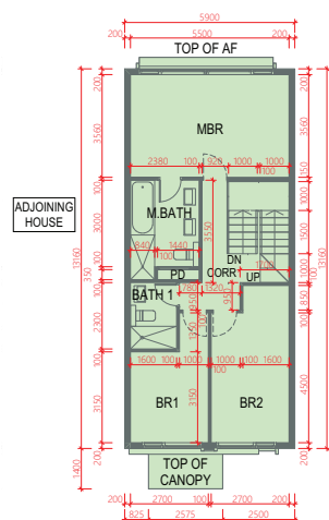
FIRST FLOOR 1樓
