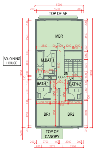
FIRST FLOOR 1樓
