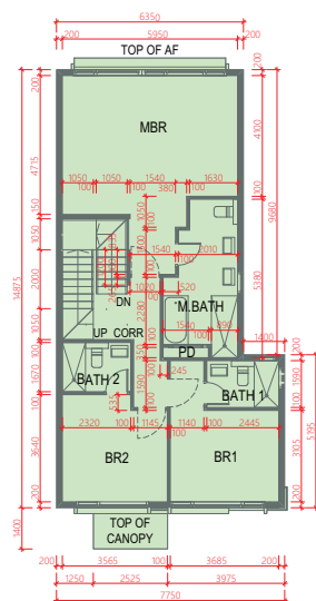
FIRST FLOOR 1樓
