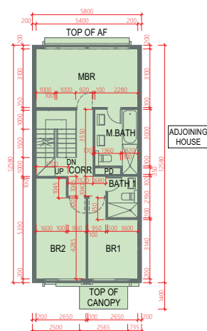
FIRST FLOOR 1樓
