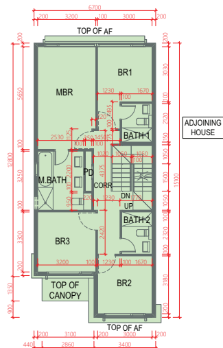
FIRST FLOOR 1樓
