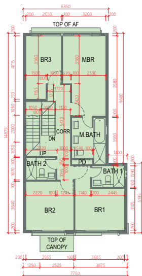
FIRST FLOOR 1樓
