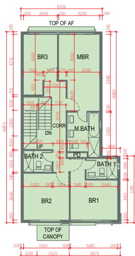
FIRST FLOOR 1樓
