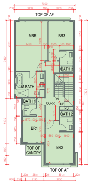
FIRST FLOOR 1樓
