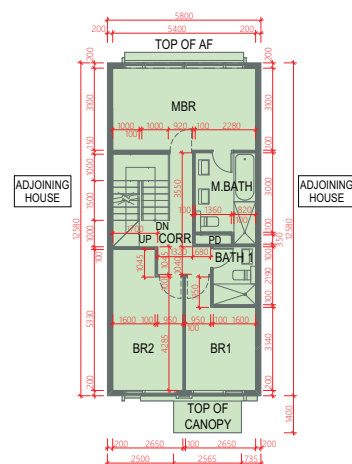
FIRST FLOOR 1樓
