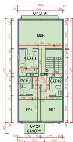
FIRST FLOOR 1樓
