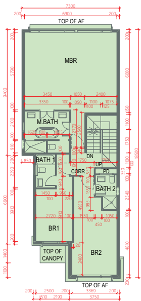
FIRST FLOOR 1樓
