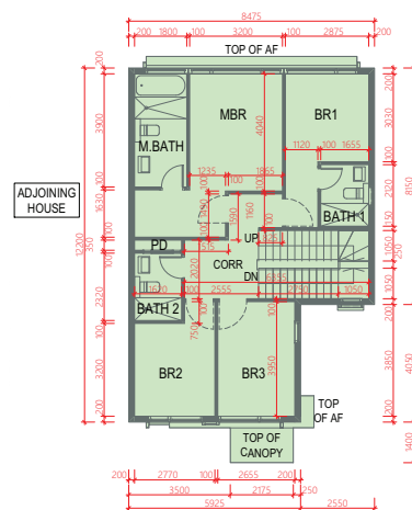
FIRST FLOOR 1樓
