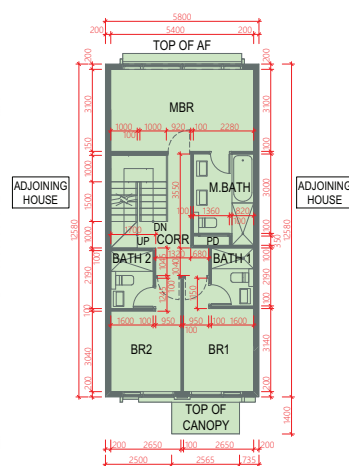
FIRST FLOOR 1樓
