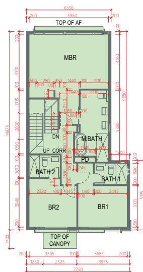
FIRST FLOOR (AS-IS PLAN) 1樓 (現狀平面圖)
