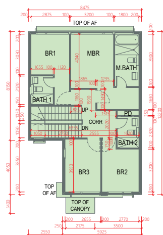
FIRST FLOOR 1樓
