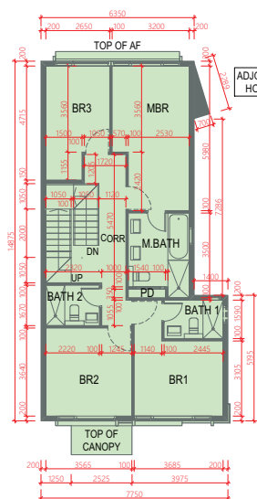
FIRST FLOOR 1樓
