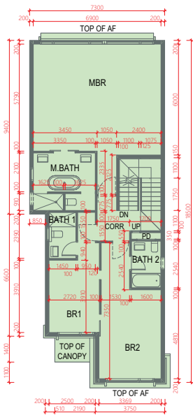
FIRST FLOOR (AS-IS PLAN) 1樓 (現狀平面圖)
