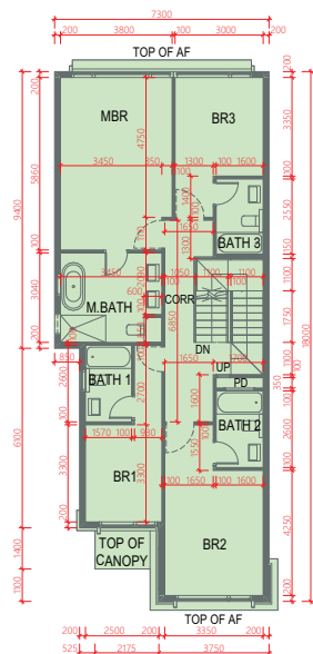
FIRST FLOOR 1樓
