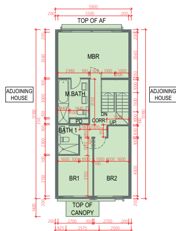
FIRST FLOOR 1樓
