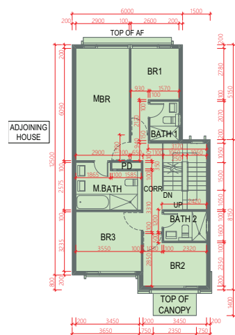
FIRST FLOOR 1樓
