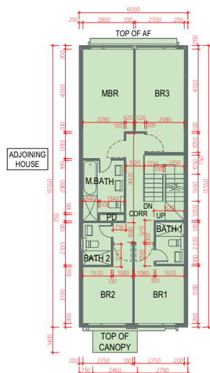
FIRST FLOOR 1樓
