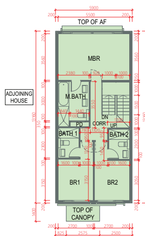
FIRST FLOOR 1樓
