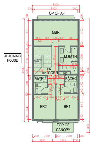
FIRST FLOOR 1樓
