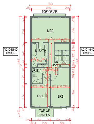
FIRST FLOOR 1樓
