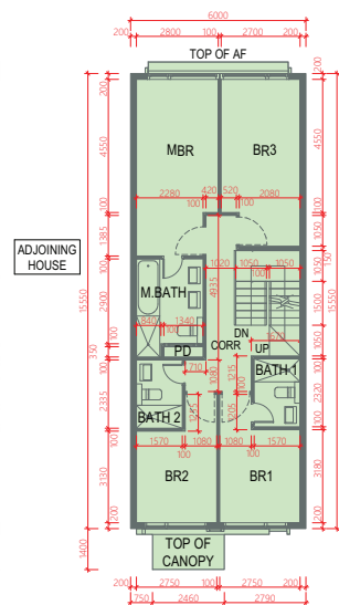
FIRST FLOOR 1樓
