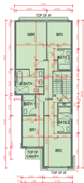
FIRST FLOOR 1樓
