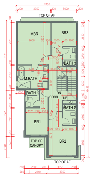
FIRST FLOOR 1樓
